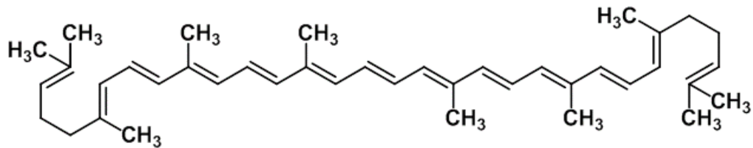
all- trans -lycophene
