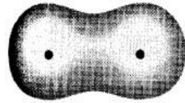
(a) \sigma orbital
