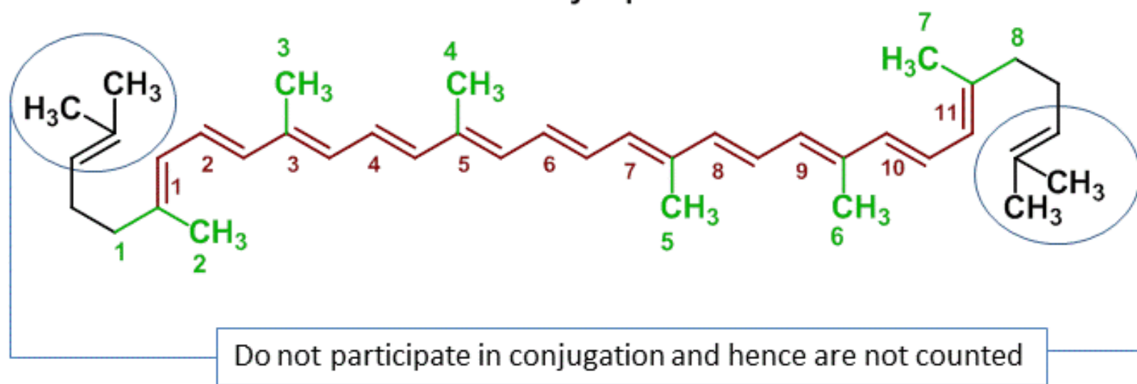
all- trans -lycophene
