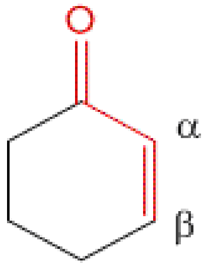
Cyclohexenone
