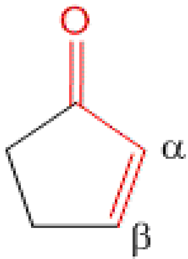
Cyclopentenone
